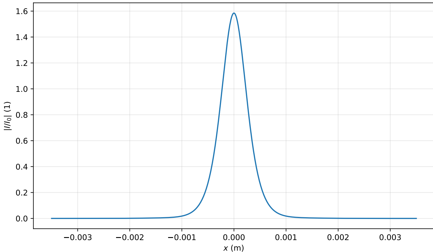
Intensity profile I(x, y = 0, z = 2.866m)/I_0 , P_{in}=0.9P_{cr} , artificial time
